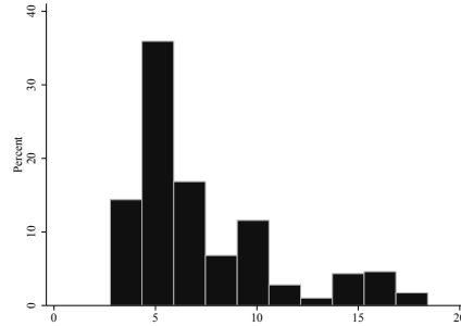
Figure C.1: Distribution of \sigma_b , 2008-2013
